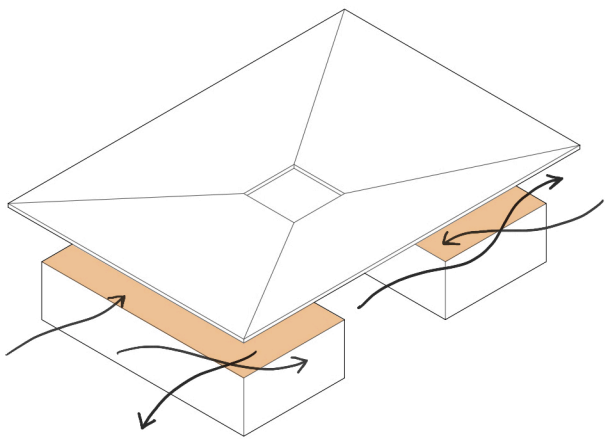
CROSSED VENTILATION
