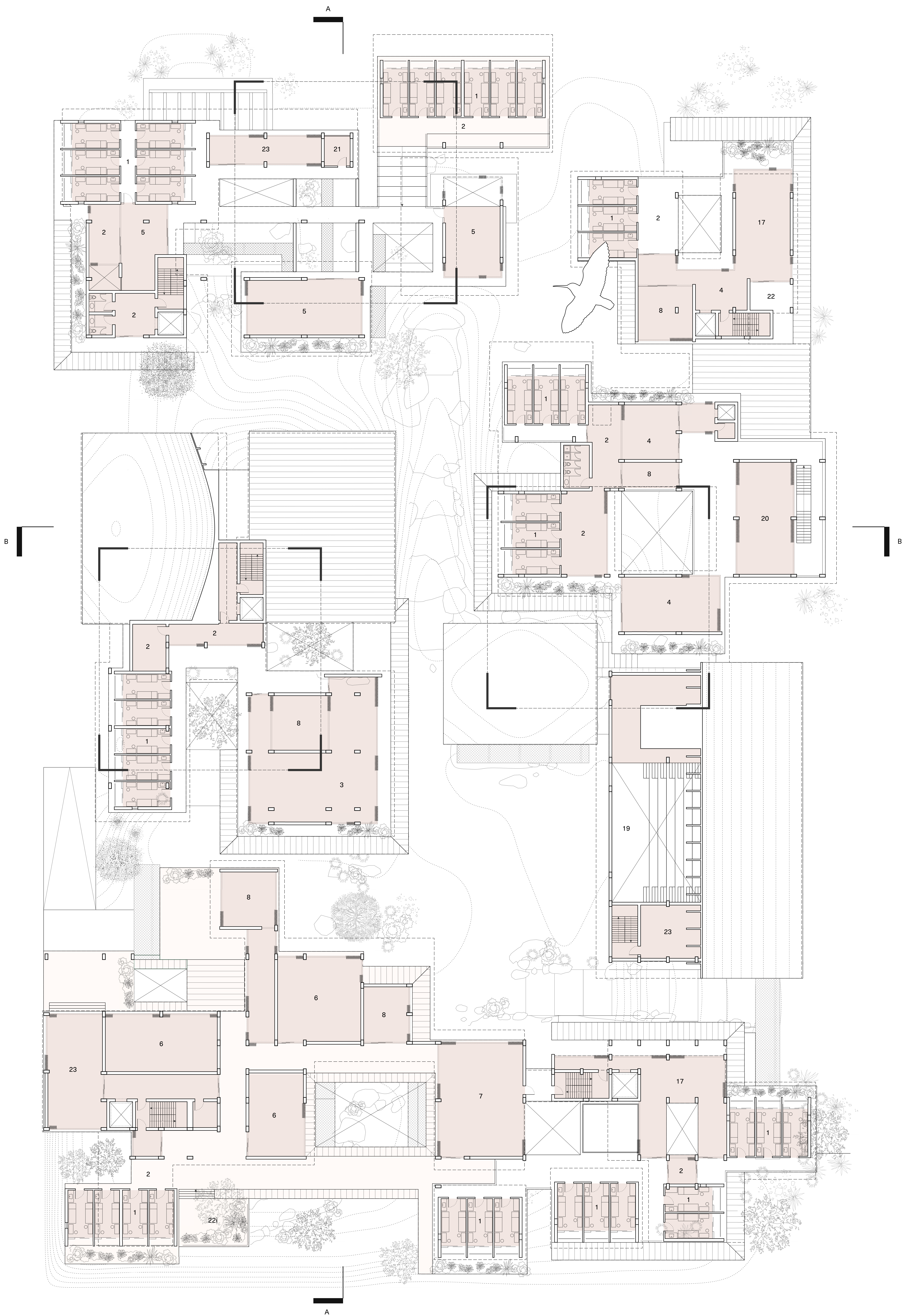
L01 Plan 3/32" = 1'-0"
