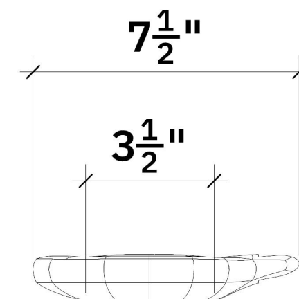
RIGHT VIEW
