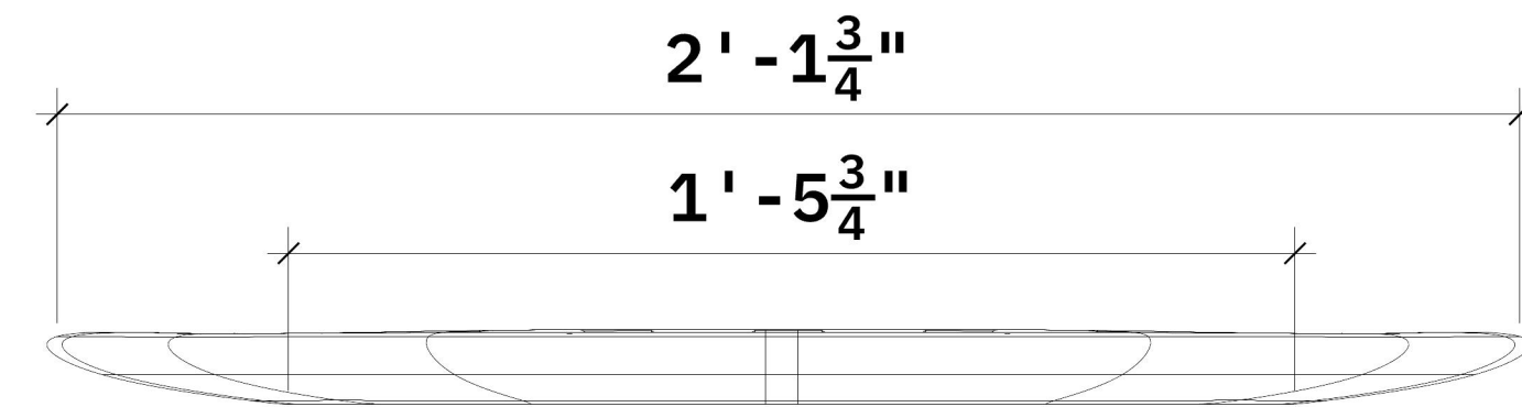
FRONT VIEW
