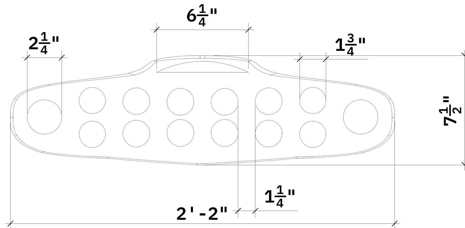
TOP VIEW
