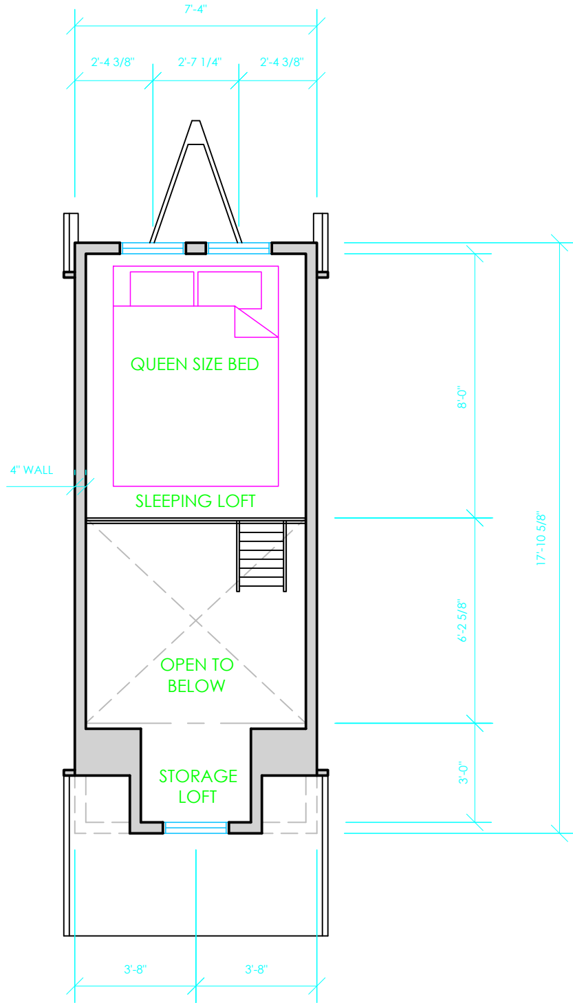
TINY HOUSE LOFT FLOOR PLAN SCALE: \frac{1}{4}" = 1'-0" ANNABELLE WARNER IDES 240 SPRING SEMESTER 2024
