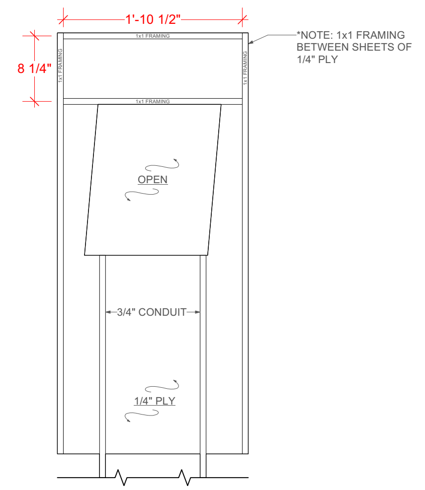
3 BUS UNIT INTERNAL STRUCTURE ELEVATION Scale: 1" = 1'-0"
