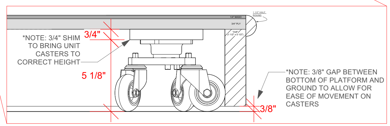
5 CASTER BUILD DETAIL Scale: 3" = 1'-0"
