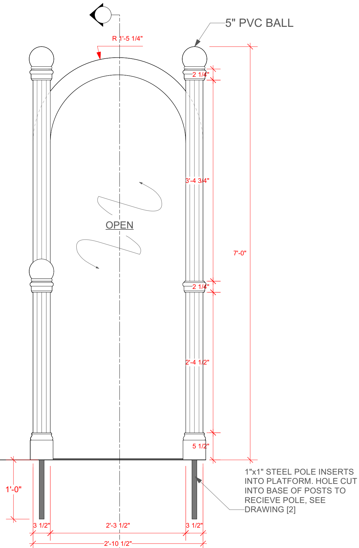
SIDE (SR)
