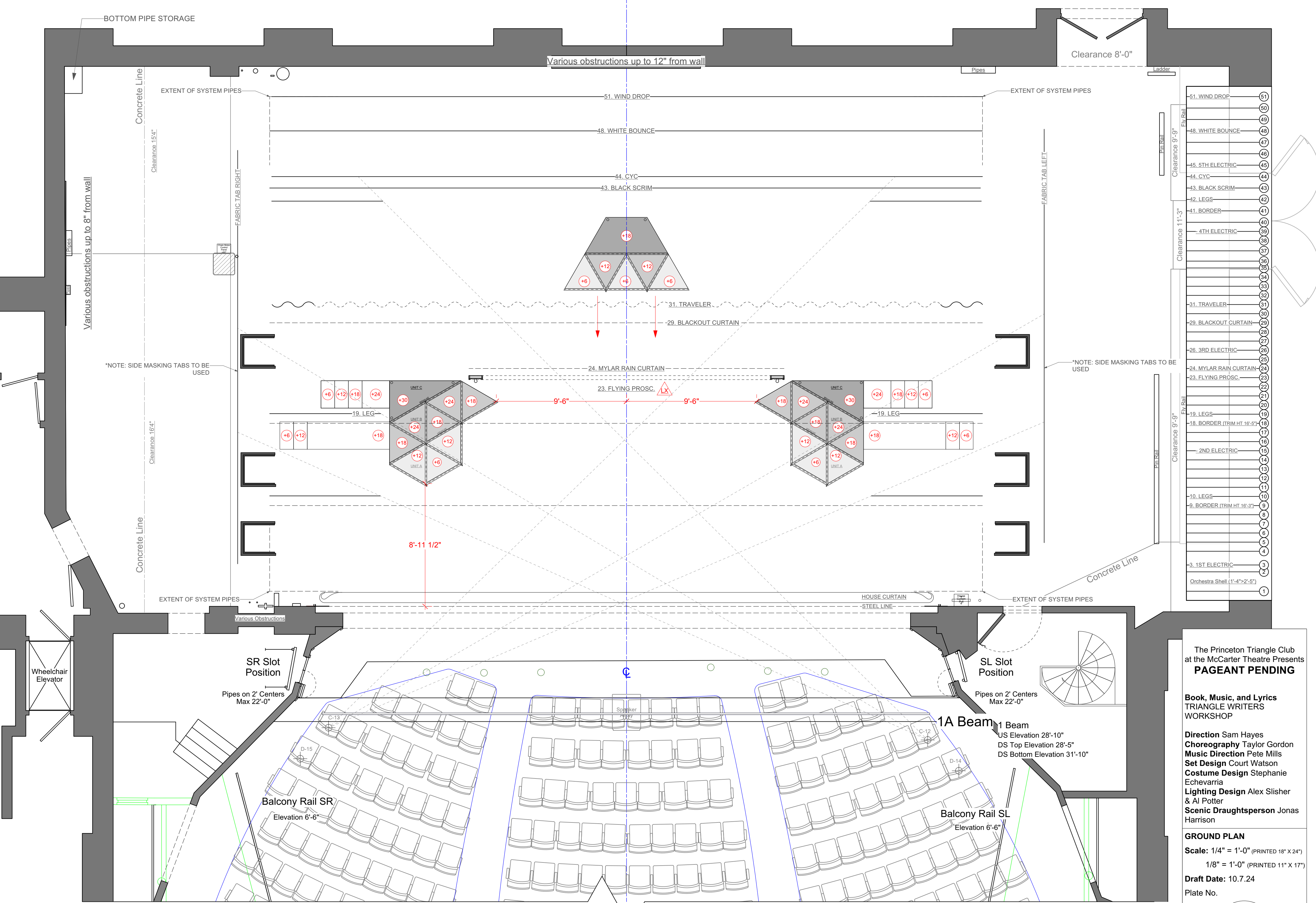
1 1/4" GROUND PLAN Scale: 1/4" = 1'-0"
