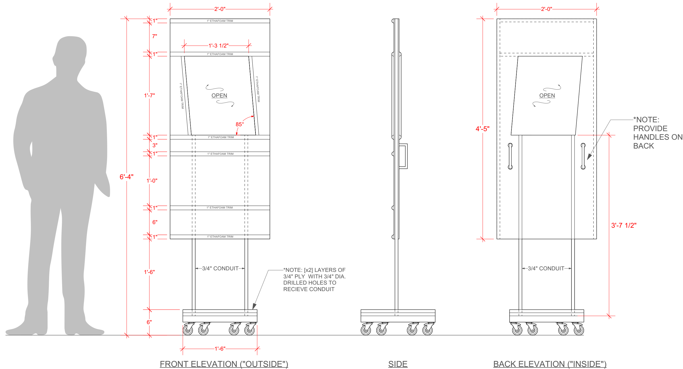
FRONT ELEVATION ("OUTSIDE")
