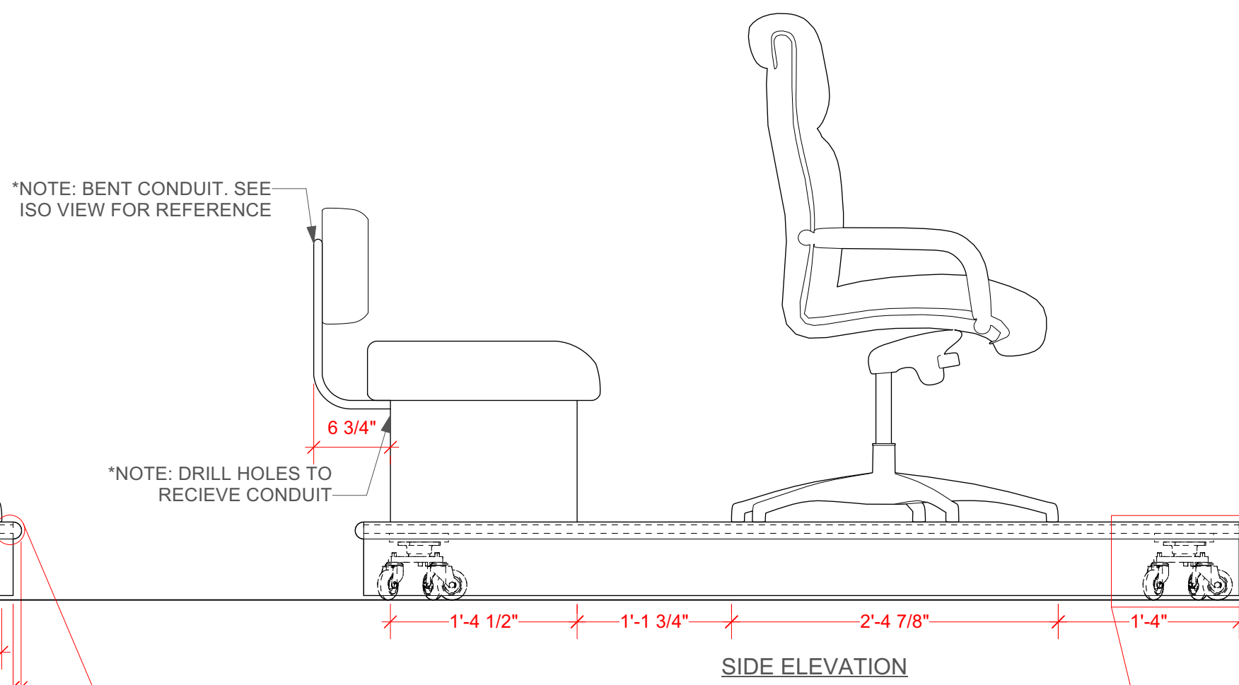
1 CAR UNIT ELEVATION Scale: 1" = 1'-0"
