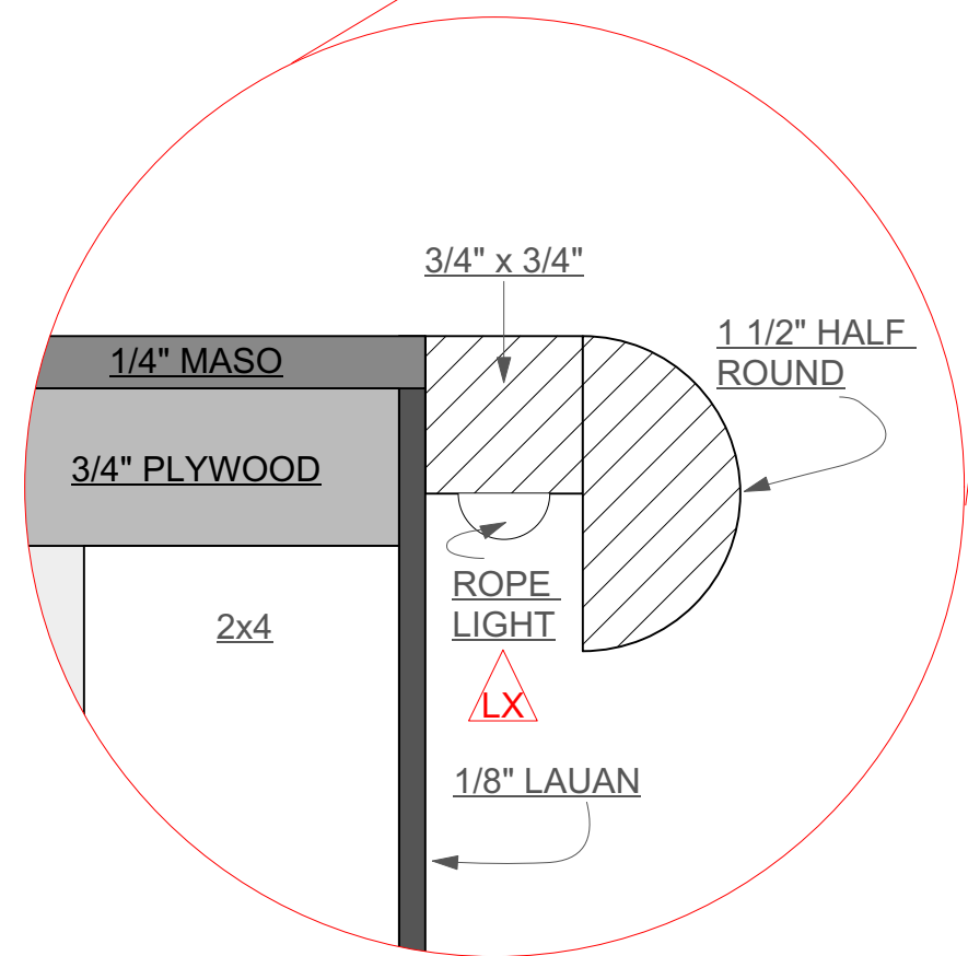
3 PLATFORM BUILD DETAIL Scale: Actual Size
