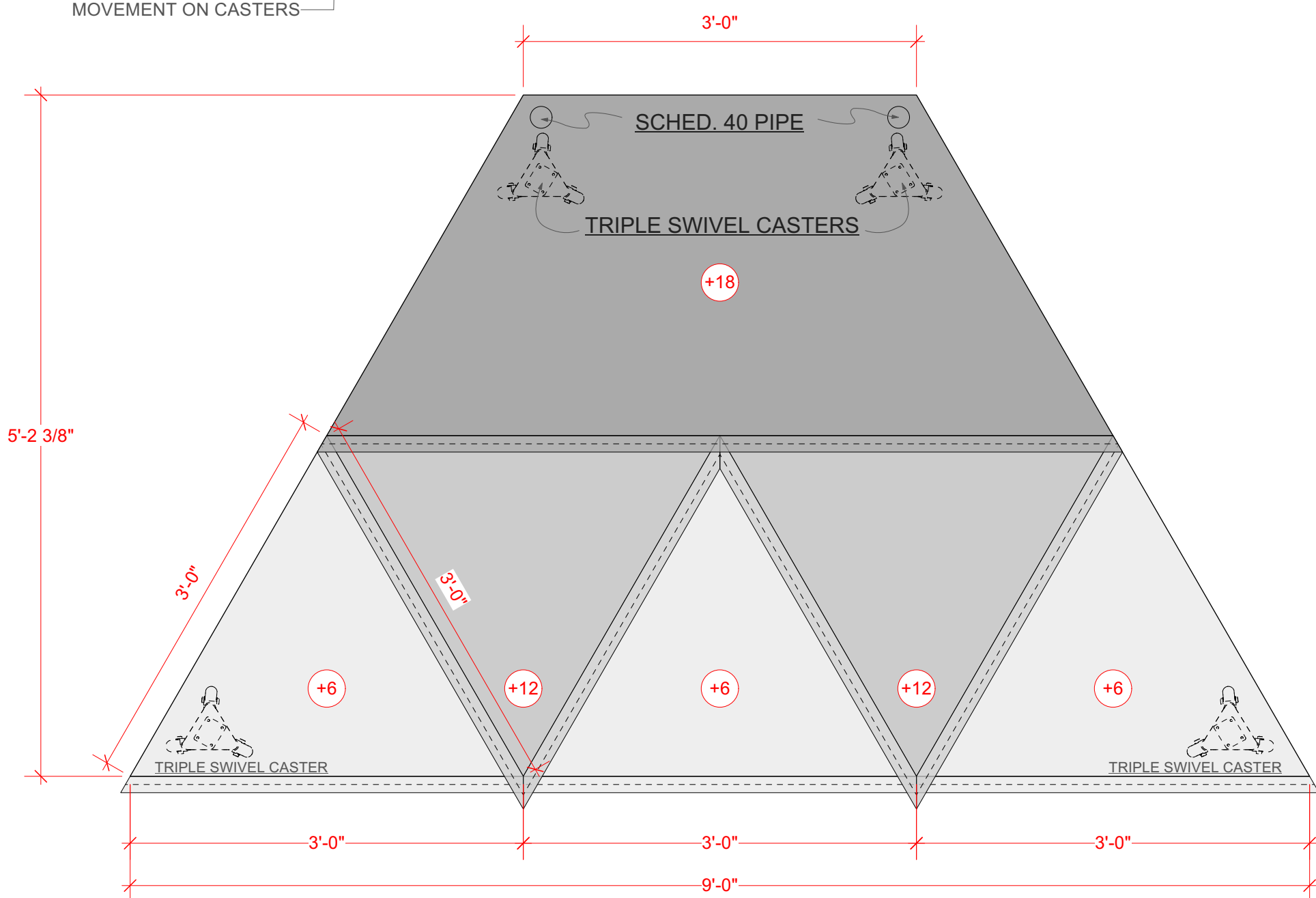
PLAN
