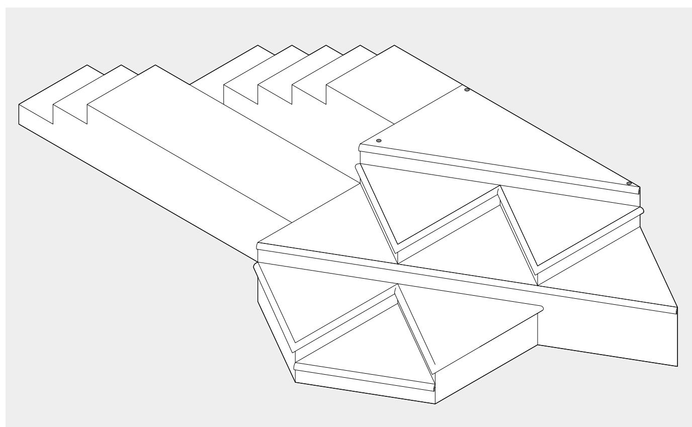
3 SR PLATFORM ISOMETRIC VIEW Scale: 1/2" = 1'-0"
