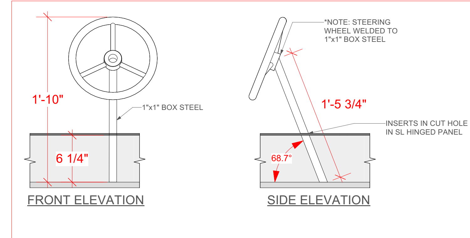
2 STEERING WHEEL UNIT ELEVATION Scale: 1 1/2" = 1'-0"
