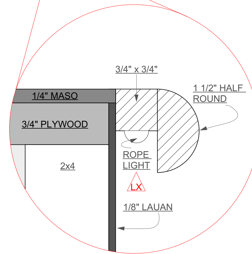
2 PLATFORM BUILD DETAIL Scale: Actual Size
