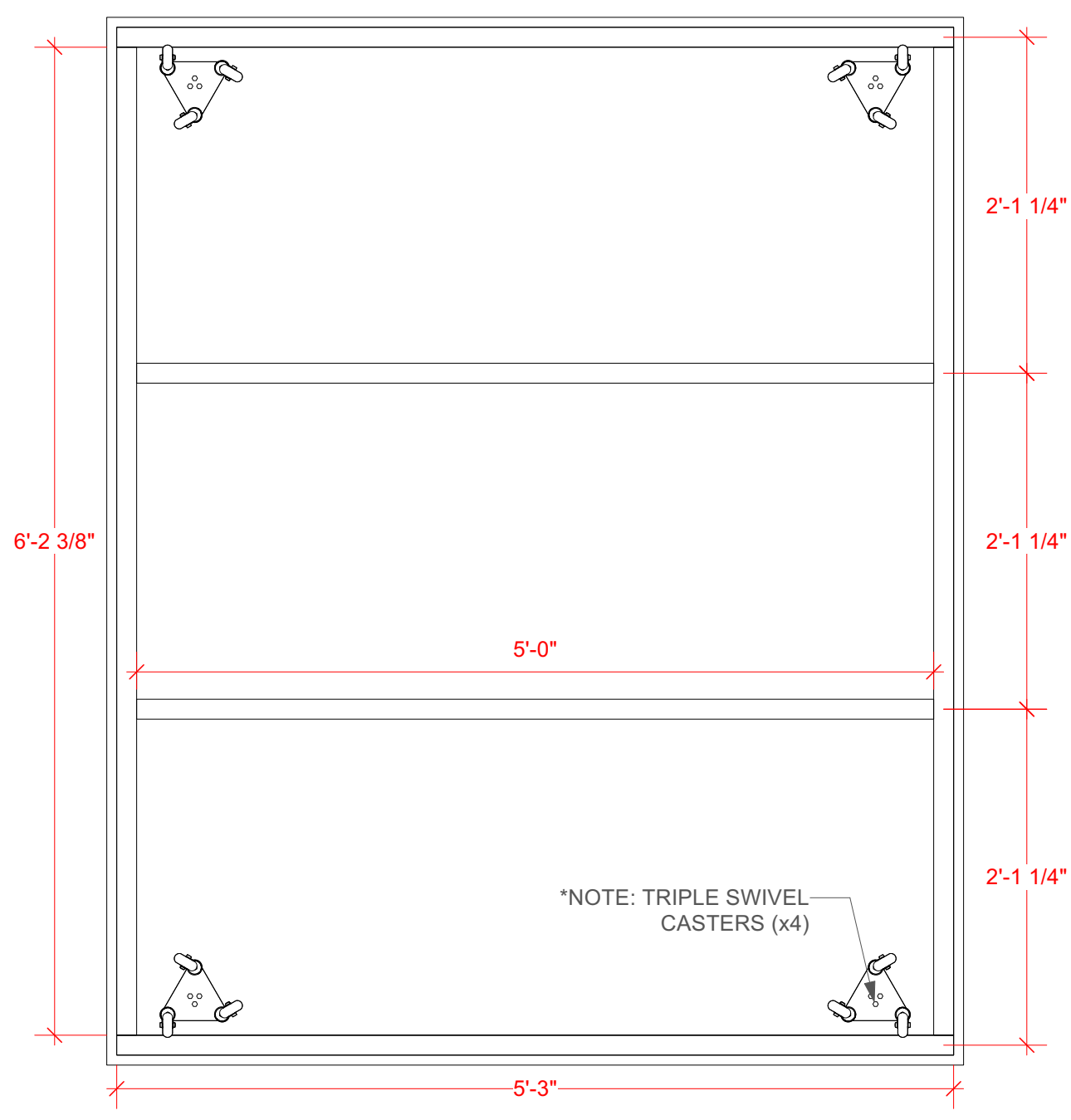
2 [CAR] PLATFORM UNDERSIDE ELEVATION Scale: 1" = 1'-0"
