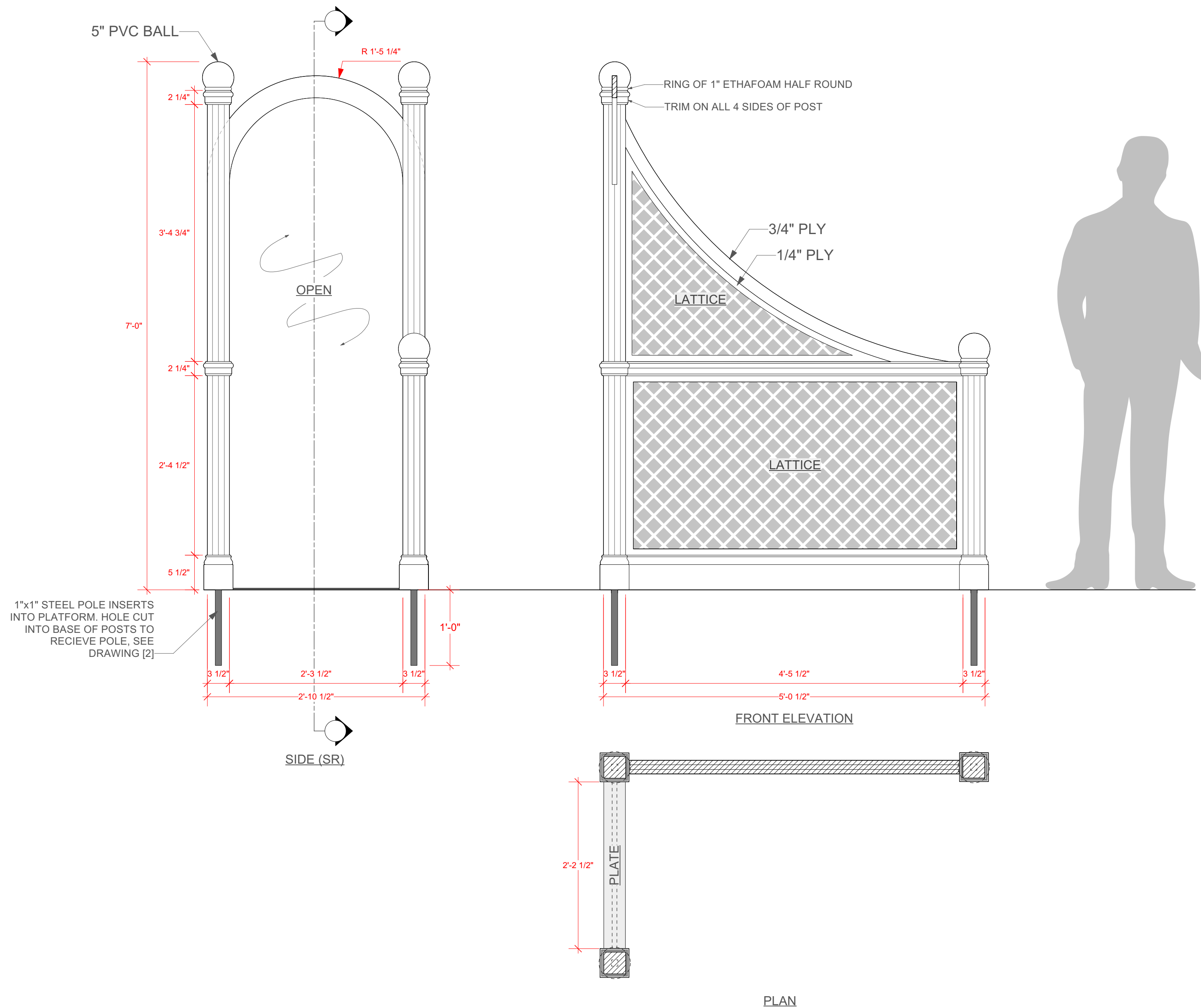
1 SR PAGEANT WALL UNIT ELEVATION Scale: 1" = 1'-0"
