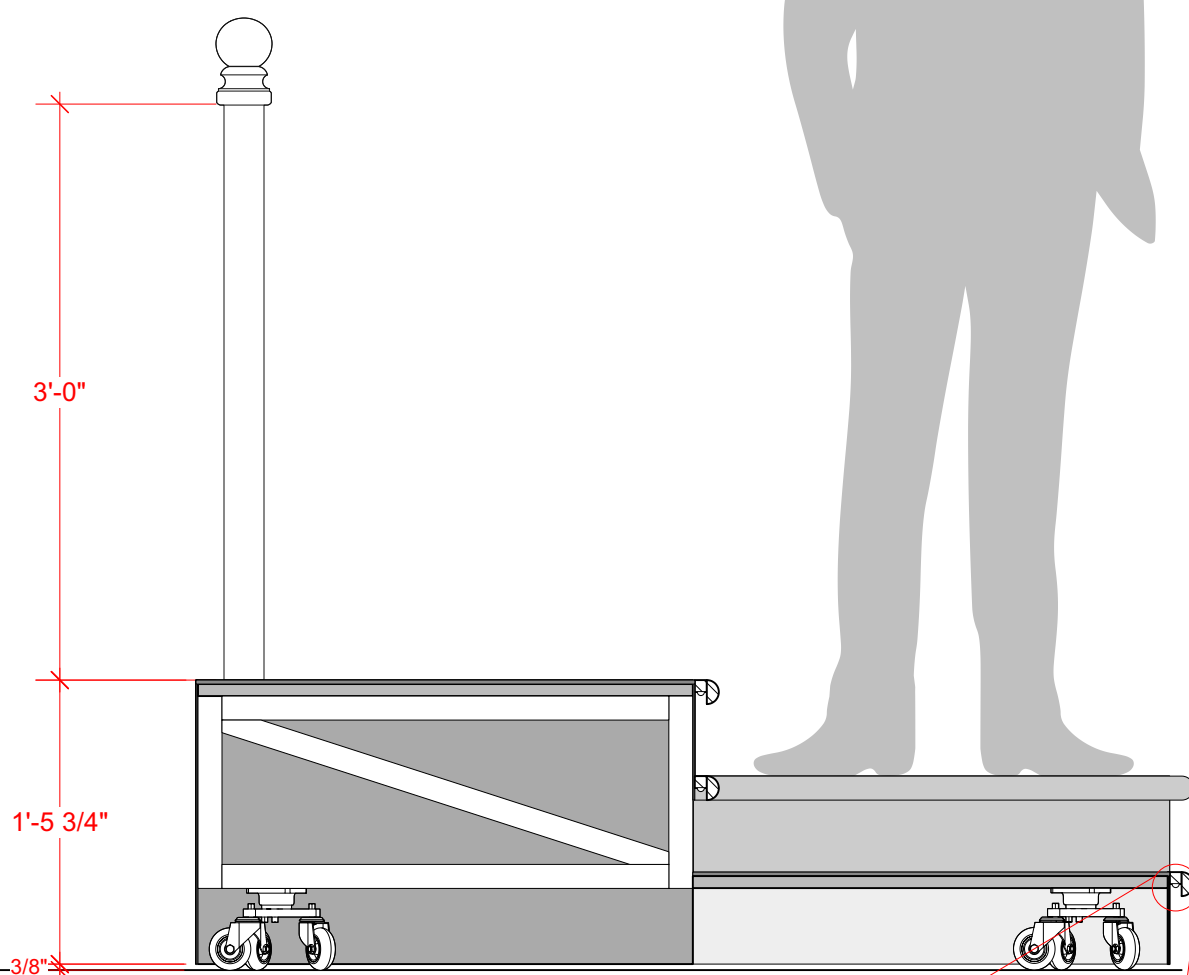
SECTION
