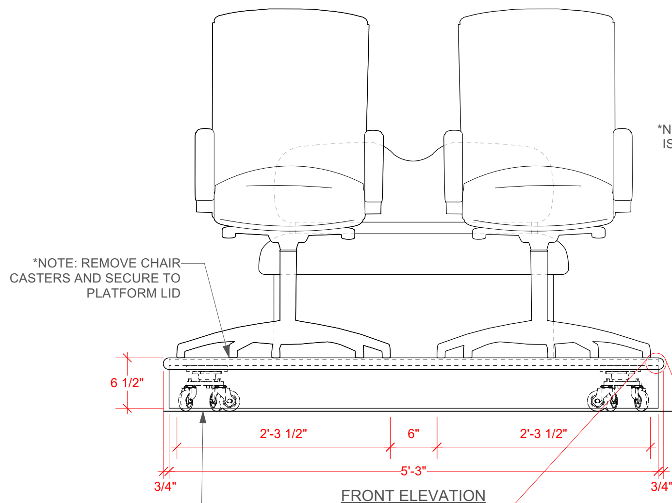
FRONT ELEVATION
