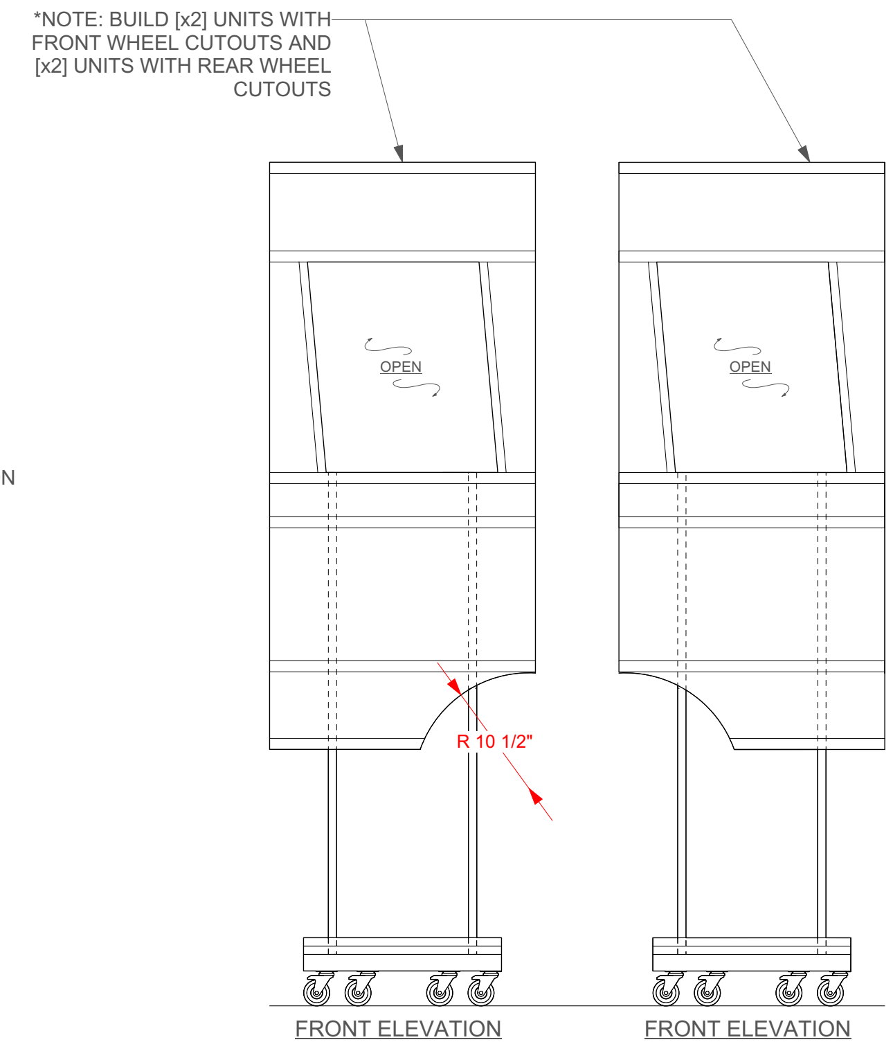
FRONT ELEVATION
