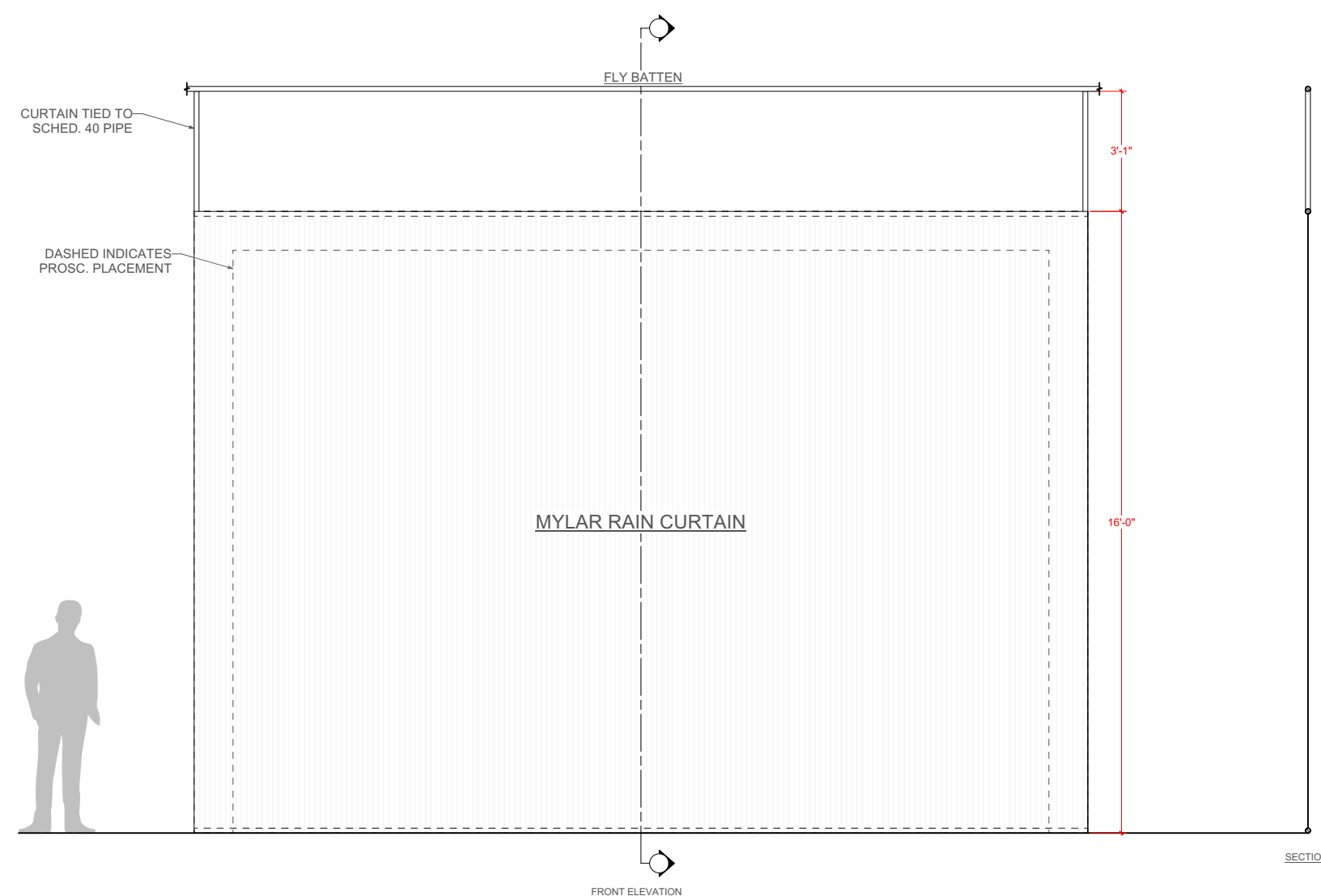
2 RAIN CURTAIN ELEVATION Scale: 1/4" = 1'-0"
