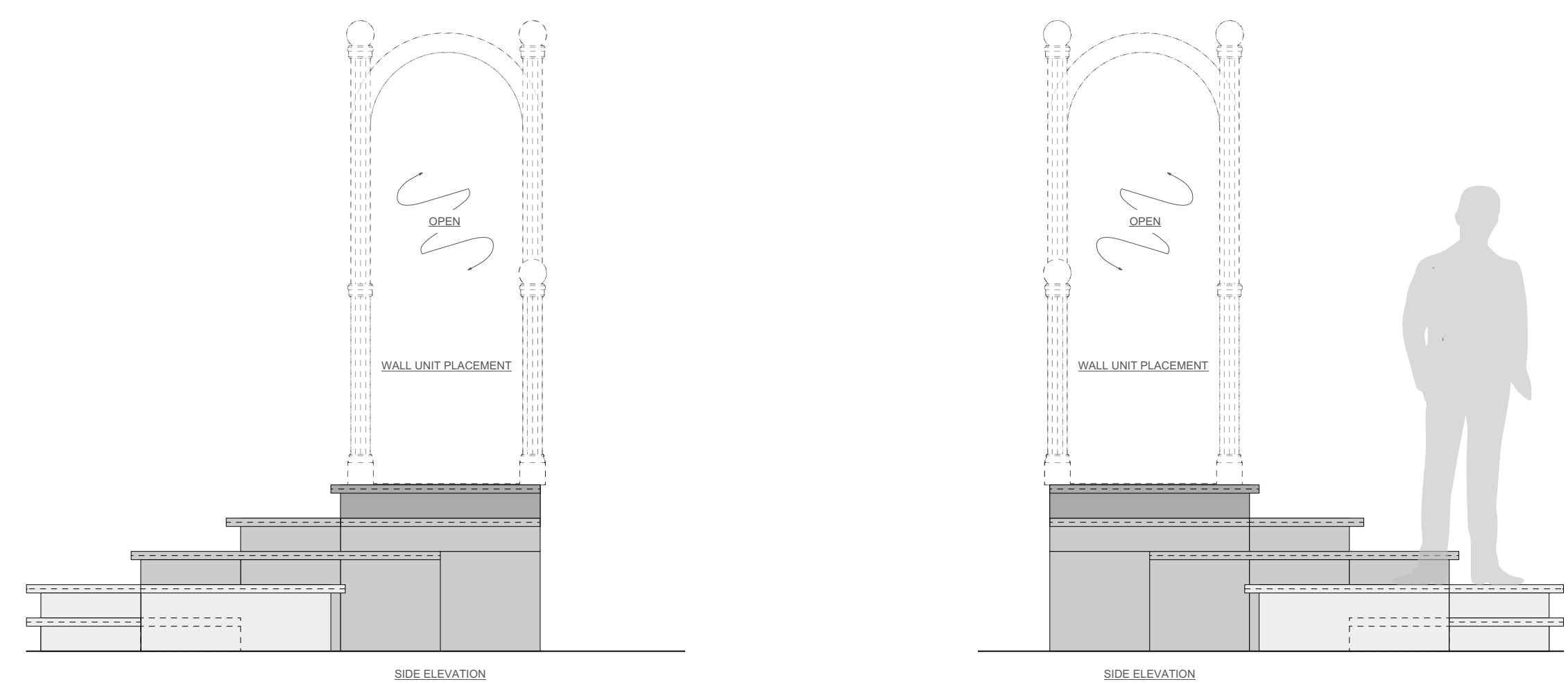
3 SL & SR PLATFORMS: SIDE ELEVATION Scale: 1/2" = 1'-0"
