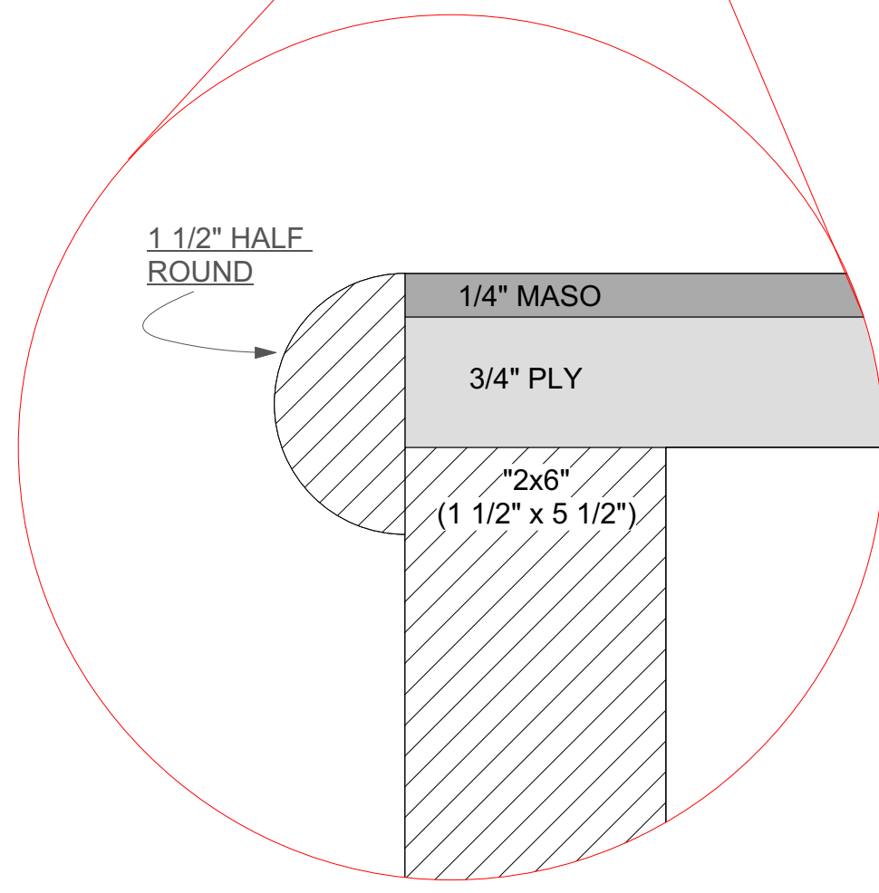
3 PLATFORM BUILD DETAIL Scale: Actual Size
