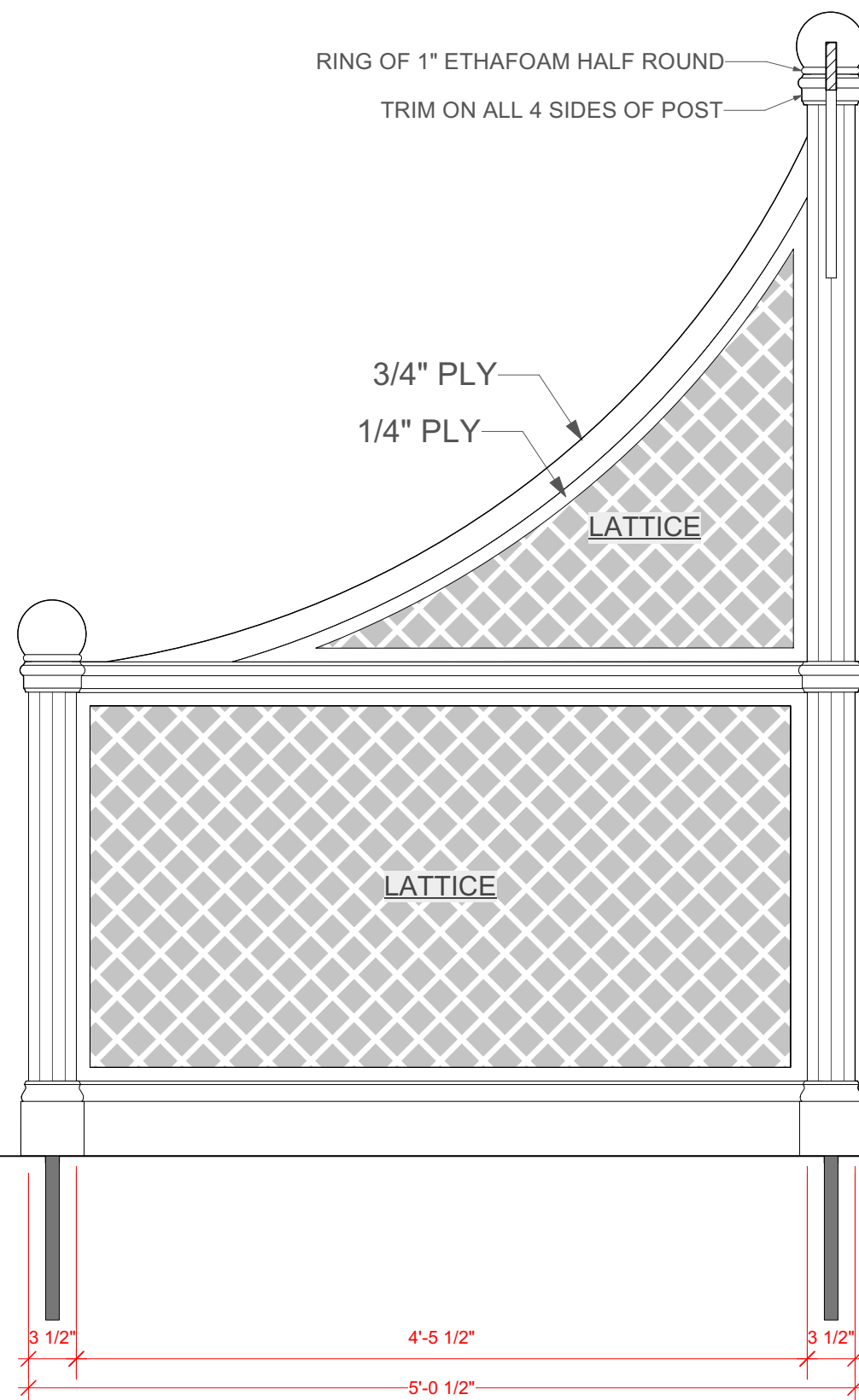
FRONT ELEVATION
