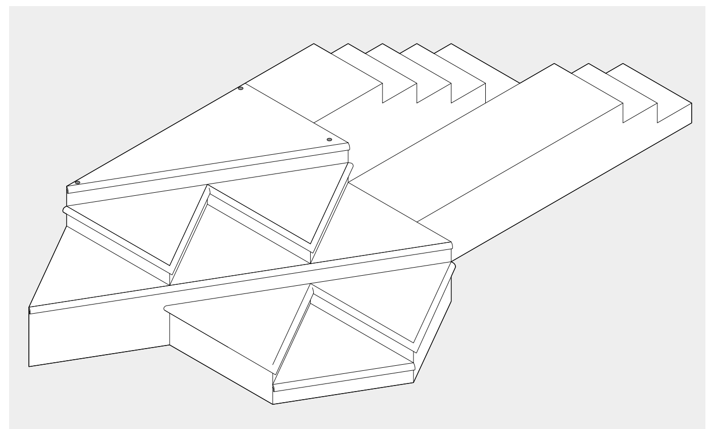
3 SL PLATFORM ISOMETRIC VIEW Scale: 1/2" = 1'-0"
