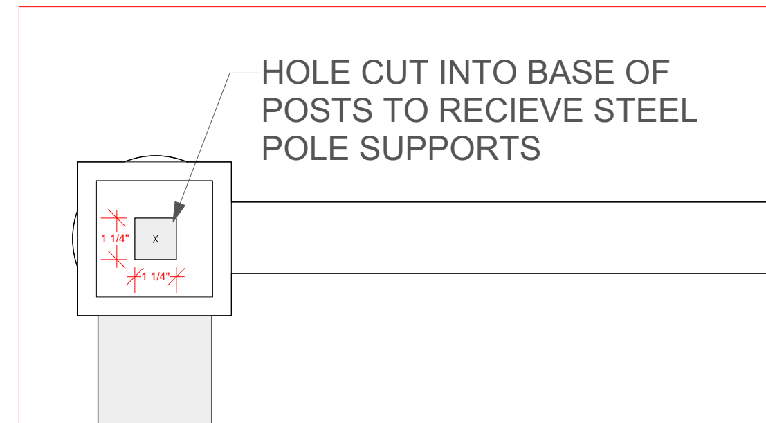
2 POST UNDERSIDE ELEVATION Scale: 3" = 1'-0"
