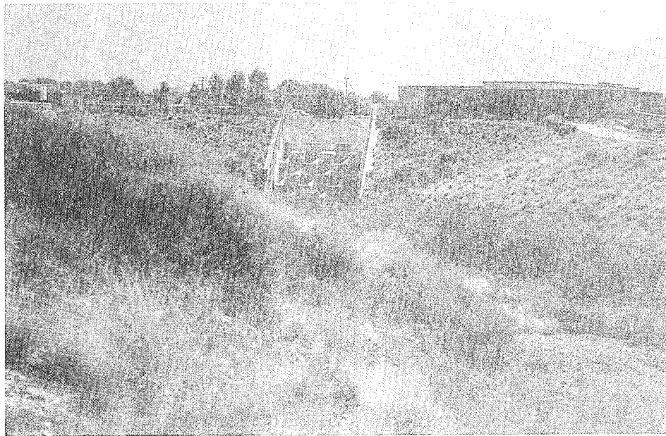
Figure 6. Bear Canyon Arroyo drop structures upstream from confluence with North Diversion Channel
