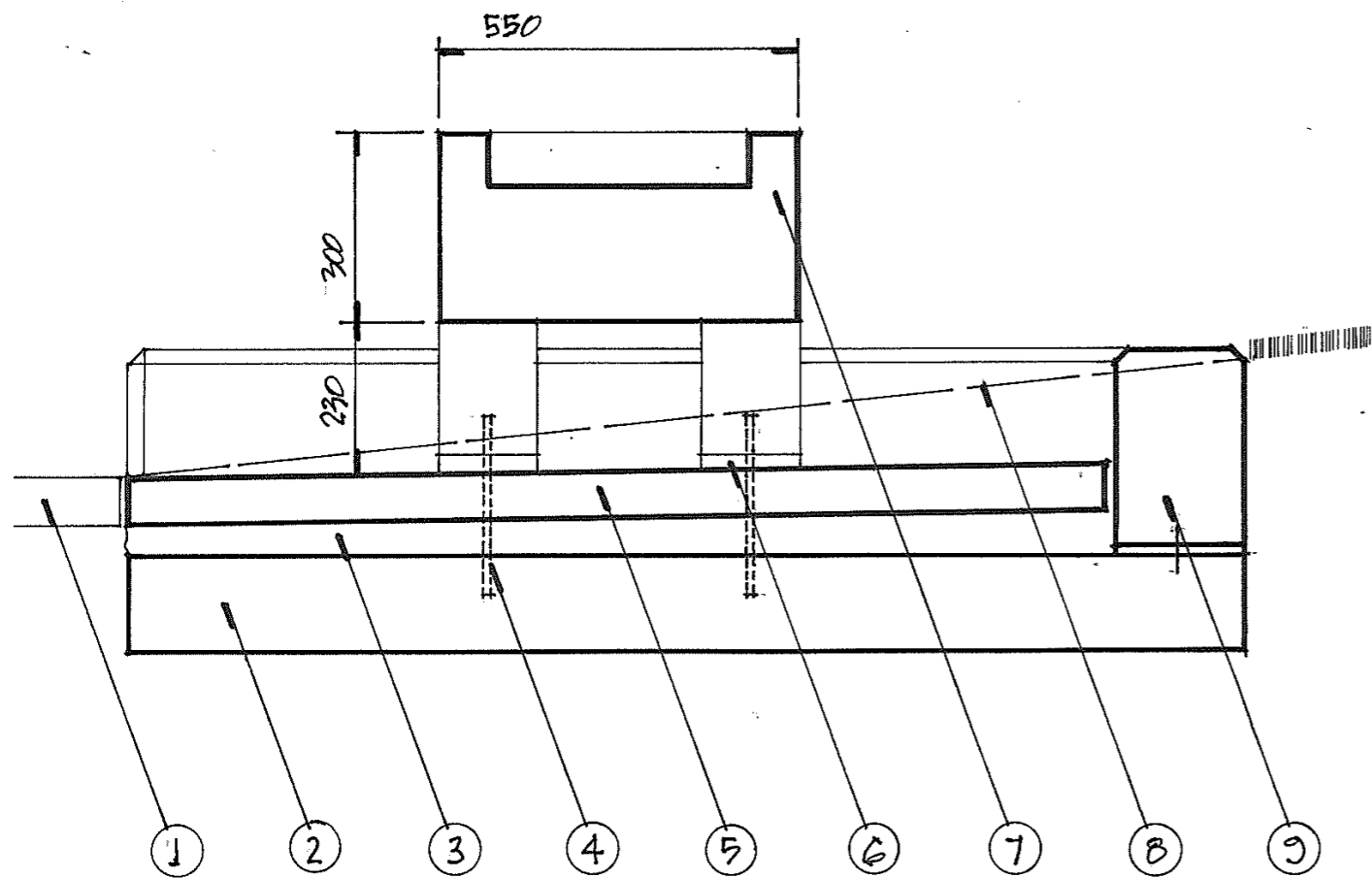
SECTION Scale 1:10' @ A4 BIRD BATH
